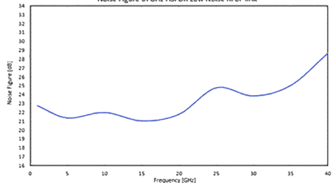
Noise Figure 67GHz HSFDR Low Noise RToF link
