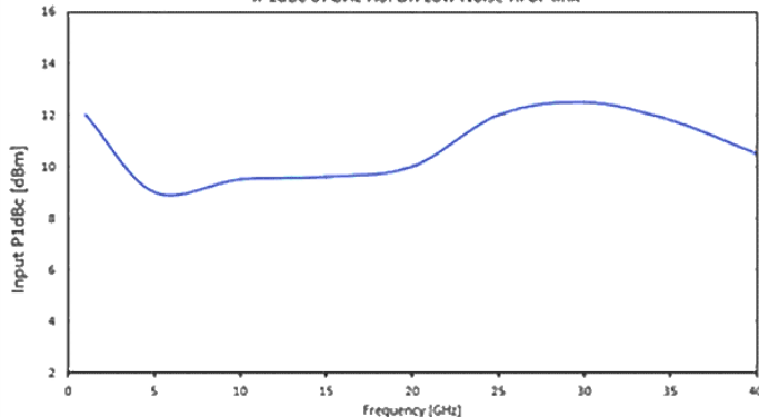
IP1dBc 67GHz HSFDR Low Noise RToF link
